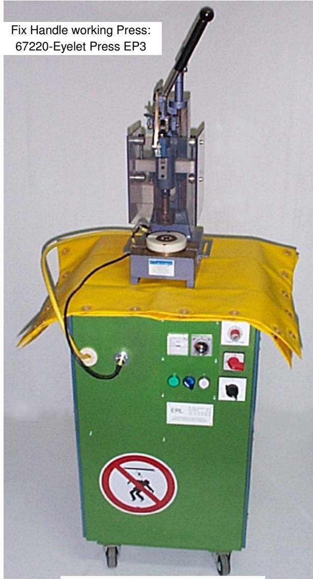
HF Generator 1500wHF model: Ref: 67220-Gen 3000 Eyelets M
